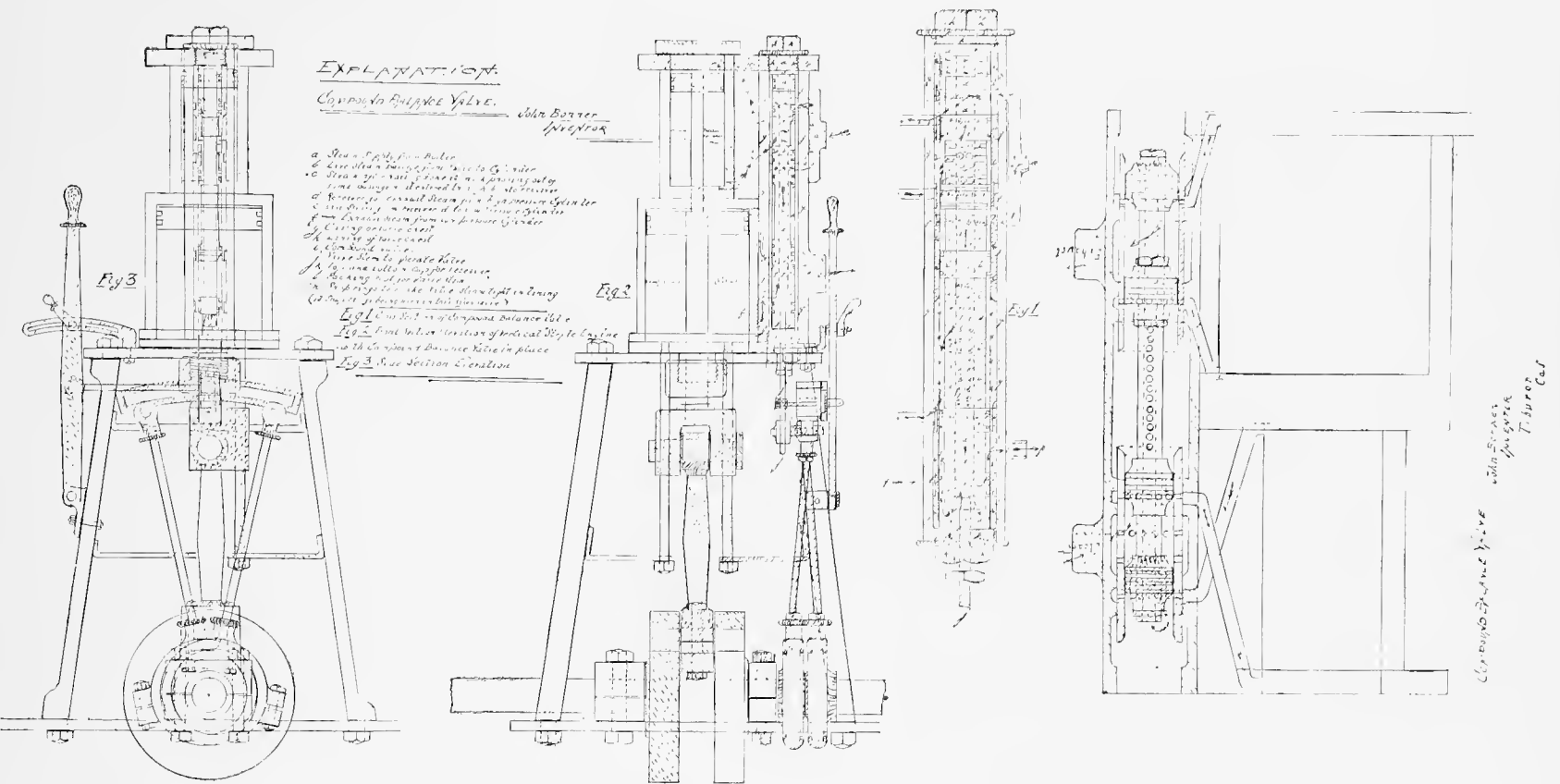
BONNER'S PATENT BALANCE VALVE.—Designed by John Bonner, Tiburon, Cal.
